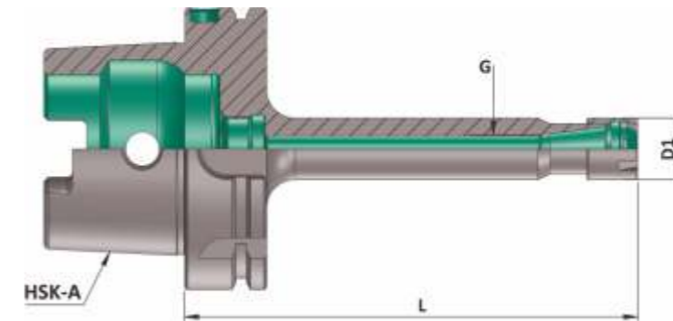
HSK-A (DIN 69893-1) Collet Chuck ER-M Type
