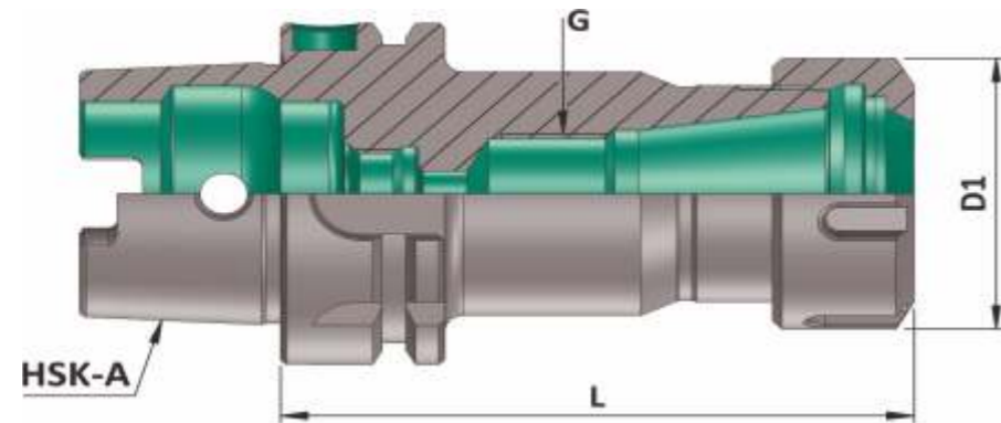
HSK-A (DIN 69893-1) Collet Chuck (ER)
