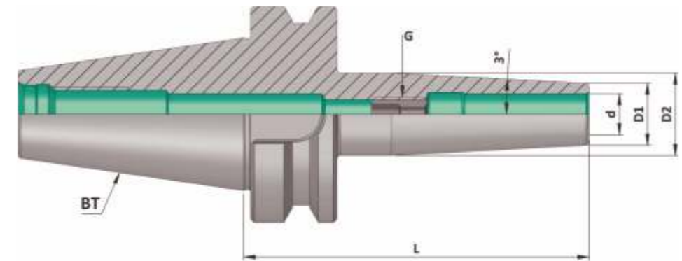
BT (MAS 403) (SFH SLIM 3°) (AD) JD
