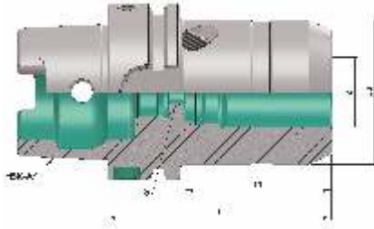
HSK-A (DIN 69893 - 1) Hydraulic Expansion Chuck
