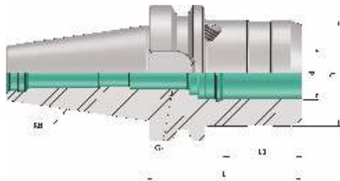
BBT (MAS 403) Hydraulic Expansion Chuck (AD)
