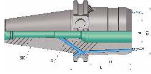
SK (DIN 69871) Hydraulic Expansion Chuck (FCC - AD+B)
