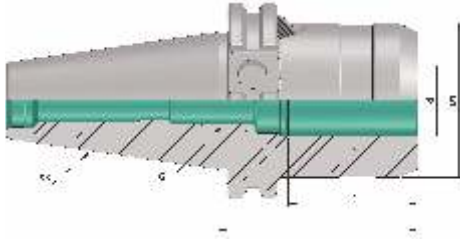
SK (DIN 69871) Hydraulic Expansion Chuck (AD)
