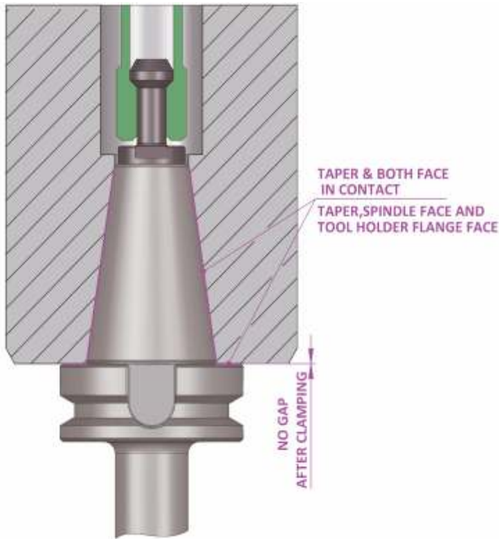
BBT (BT MAS 403) TAPER AND BOTH FACE CONTACT HOLDER (After Clamping)
